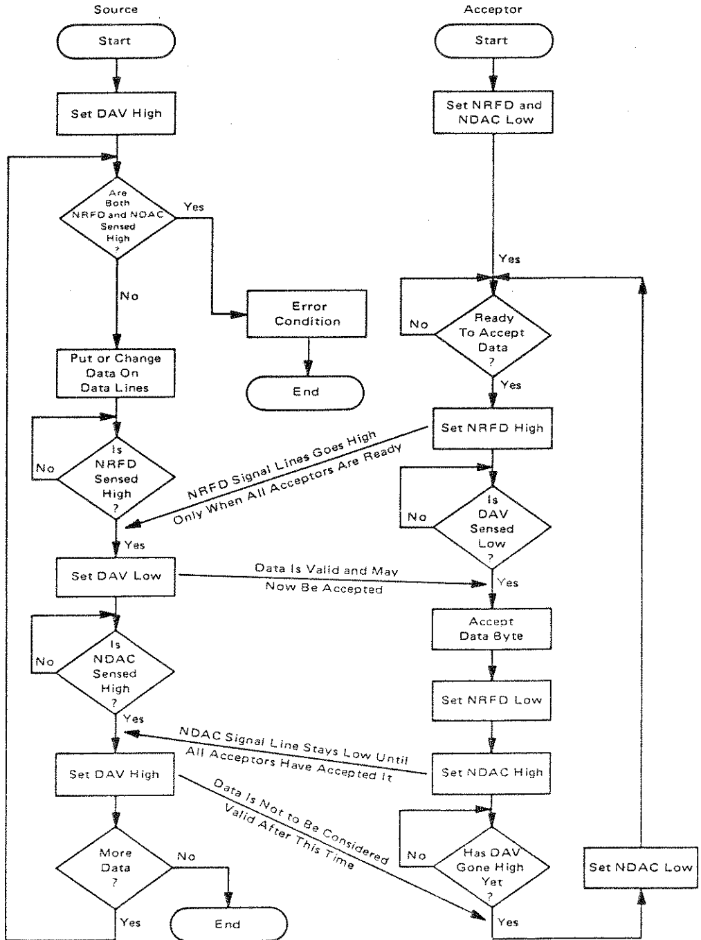
Flow diagram outlines sequence of events during transfer of data byte. More than one listener at a time can accept data because of logical-AND connection of NRFD and NDAC lines.
