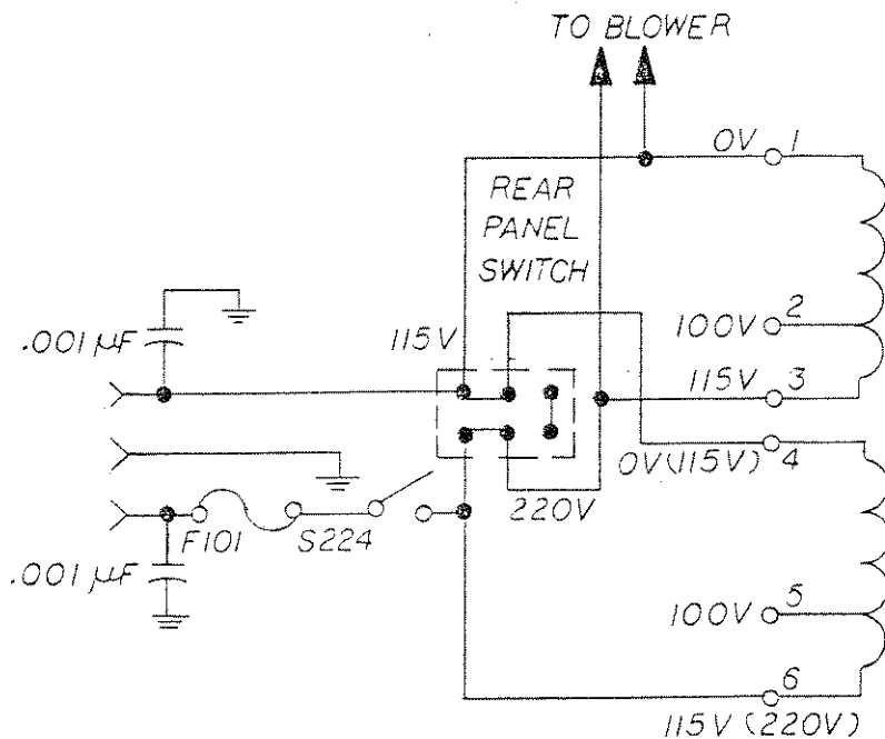
FIGURE 2-1 INPUT POWER CONNECTIONS
